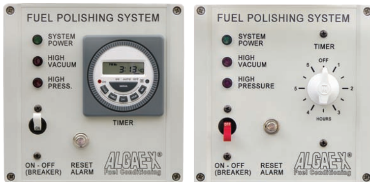
SMART FPS DX-D Digital Programmable Interface
